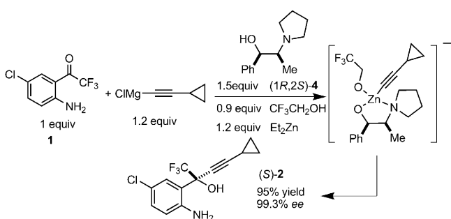
Scheme 1. Current “stoichiometric” synthesis of (S)-2, a key intermediate in the synthesis of efavirenz.
