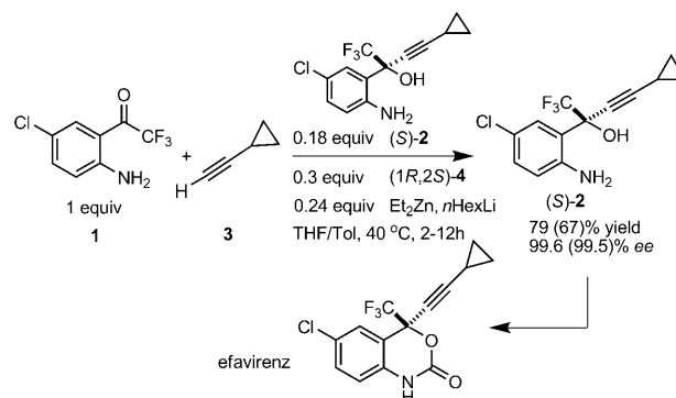
Scheme 2. Enantioselective synthesis of efavirenz by means of the autocatalytic formation of the key intermediate (S)-2.
