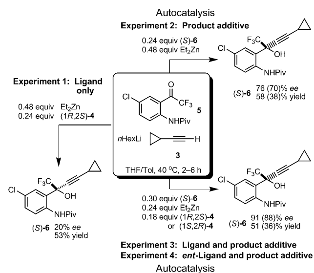
Scheme 3. Addition of alkyne 3 to N -pivaloyl-protected 5 .
